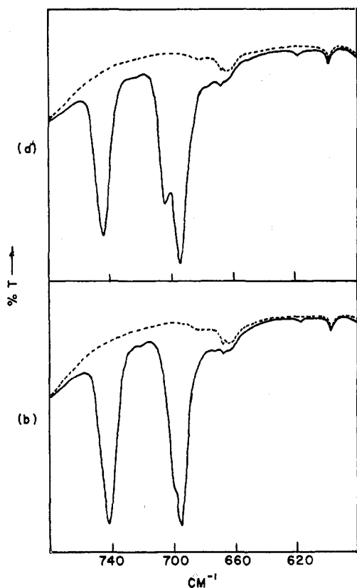
Figure 5.—Infrared spectra of \text{Ni}(\text{CO})_3\text{P}(\text{C}_6\text{H}_5)_3 and \text{P}(\text{C}_6\text{H}_5)_3 in cyclohexane, 580–780 \text{cm}^{-1} : (a) \text{Ni}(\text{CO})_3\text{P}(\text{C}_6\text{H}_5)_3 , (b) \text{P}(\text{C}_6\text{H}_5)_3 .
