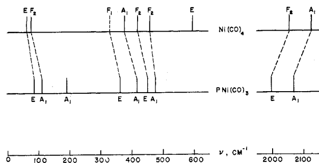
Figure 6.—Correlation of the fundamental frequencies for \text{Ni(CO)}_4 and the \text{PNi(CO)}_3 group.
