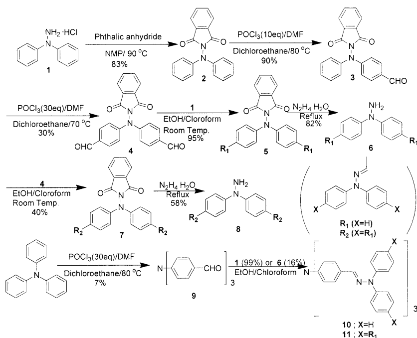
Scheme 1. Synthesis of Dendrons and Dendrimers.
