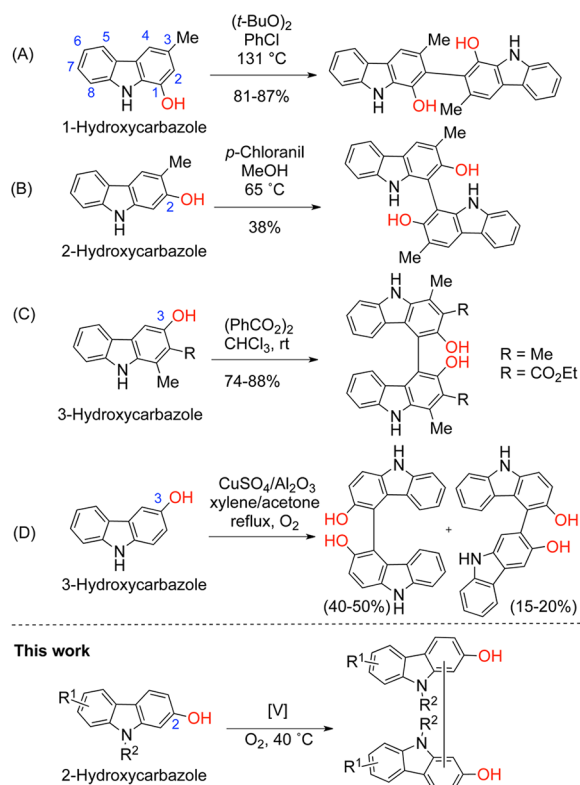
Scheme 1. Approaches to Bis(hydroxycarbazoles)
