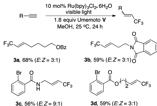
Scheme 3. Hydrotrifluoromethylation of Alkynes
