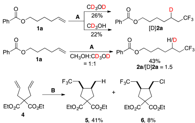
Scheme 4. Mechanistic Investigations
