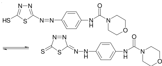
Fig. 4. Tautomerism of new 1,3,4-thiadiazole compounds
