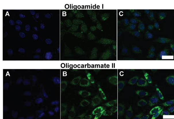
Figure 5. Confocal microscopy images of CHO-K1 cells after 4 h incubation at 37 °C with the oligoamide I (10 \mu M) and oligocarbamate II (5 \mu M). (A) Staining with nuclear stain, Hoechst 33342. (B) Fluorescence image. (C) Merged images. Scale bar: 20 \mu m.
