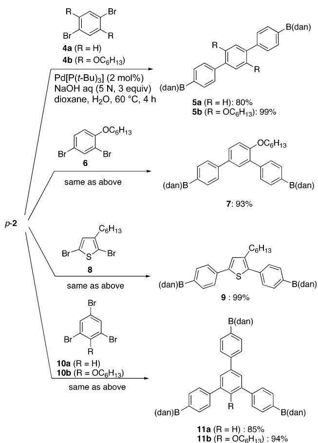
Scheme 4. Synthesis of Boron-Substituted Oligoarene Derivatives
