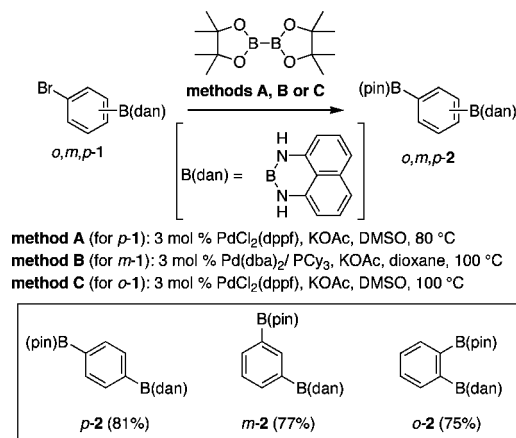
Scheme 2. Synthesis of Monoprotected Benzenediboronic Acid Derivatives
