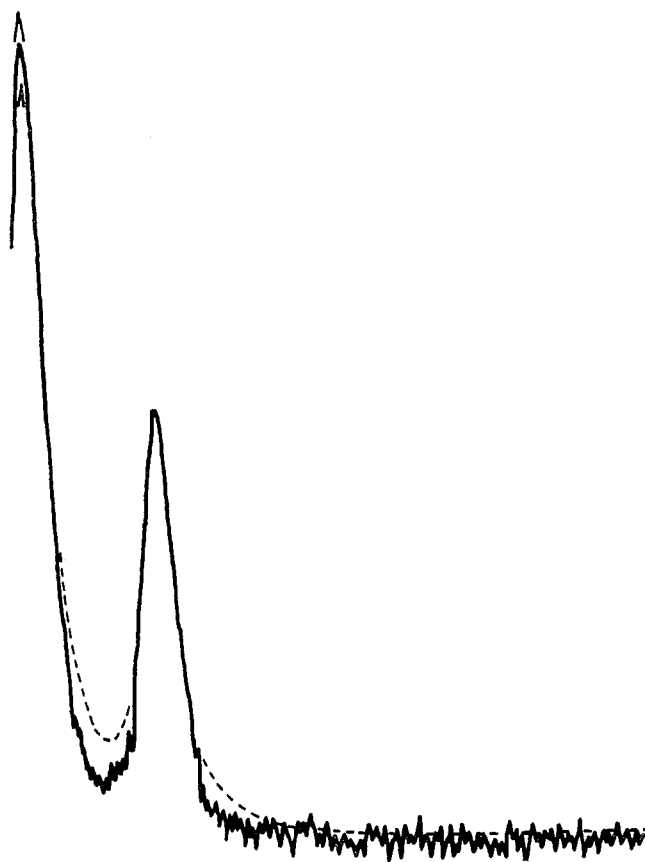
Figure 3.—Half the methylene proton resonance of trans - \text{Mo}(\text{CO})_4(\text{P}(\text{OCH}_2)_3\text{CCH}_3\text{CH}_3)_2 is shown, the tallest peak being the center. The best computed fit ( J_{\text{PP}} = 210 cps) is superimposable with the experimental curve except for the deviation (dotted line) near the base line. Using J_{\text{PP}} = 260 or 160 cps, the computed spectra differed from the best computed curve only in the higher and lower intensities for these values, respectively, of the middle peak.
