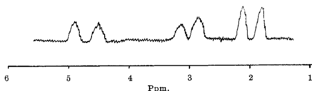
Figure 2.—Proton nmr spectrum of Fe(CO) 4 L in deuteriochloroform.
