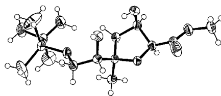
Crystal Structure of the C 10 –C 16 Tetrahydrofuran Ring 12
