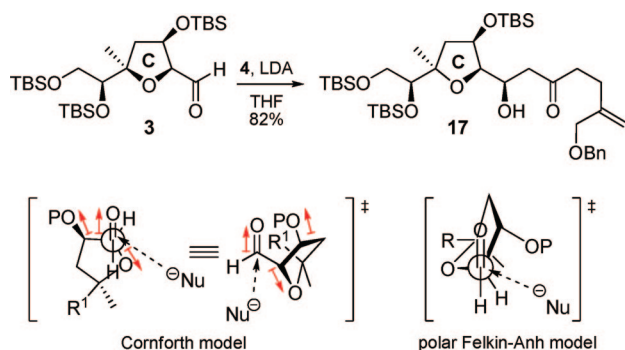
Scheme 4. Cornforth-Selective Aldol Union of 3 and 4
