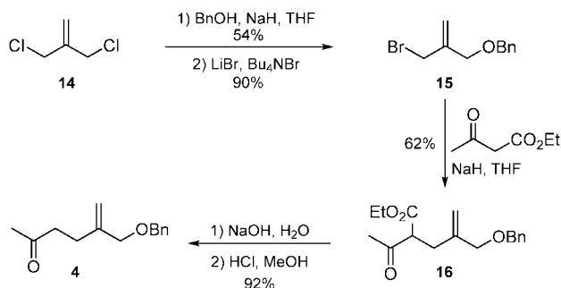
Scheme 3. Synthesis of Ketone 4
