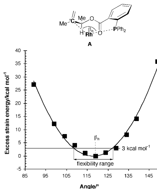
Figure 6. Relative energies of complex A as a function of the \text{C}'_{\text{olefin}}\text{-Rh-P} bite angle.
