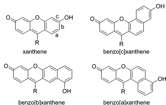
Figure 1. The xanthene dye framework and the three types of benzoxanthenes. Benzoxanthene types are each distinguished via the orientation of their naphthyl moieties.
