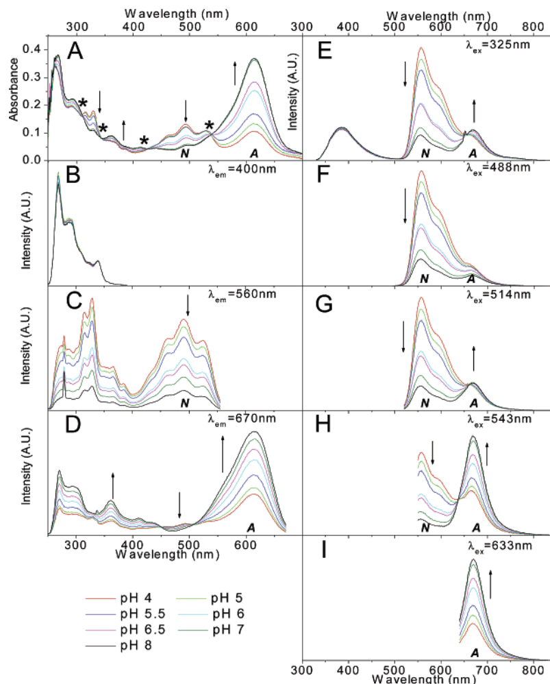
Figure 7. Spectral properties of 30 \mu M SNAFR-1 in DMSO with 0.25% phosphate buffer (50 mM) at various pH values. The trend of spectral changes is indicated by arrows as the pH increases from 4 to 8. A = anionic form; N = neutral form. (A) Absorption spectra is shown; the * in panel A indicates the positions of isosbestic points in absorbance spectra. (B–D) Excitation spectra with emission monitored at 400, 560, and 670 nm, respectively, is shown. (E–I) Data are emission spectra excited at 325, 488, 514, 543, and 633 nm, respectively, corresponding to common laser lines. All fluorescence spectra are normalized to the maximum of each data set.
