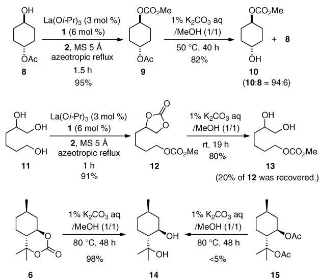
Scheme 2. Chemoselective Deprotection of Carbonates or Esters
