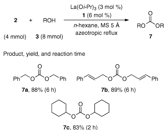
Figure 2. Double transesterification of dimethyl carbonate 2 .
