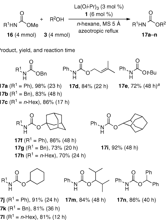
Figure 3. Transesterification of methyl carbamates 16 . Conditions: (a) t -BuOH (1 equiv) was added every 10 h, and t -BuOH (4 equiv) was used totally.
