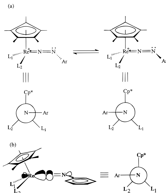
Scheme 1. (a) Idealized Conformers of [\text{Cp}^*\text{ReL}_1\text{L}_2(\text{N}_2\text{Ar})]^+ That Arise from the Two Possible Orientations of the Aryldiazenido Ligand. (b) Diagram To Show the Important Overlap of the Filled Rhenium d_\pi Orbital with the Empty In-Plane Nitrogen p Orbital
