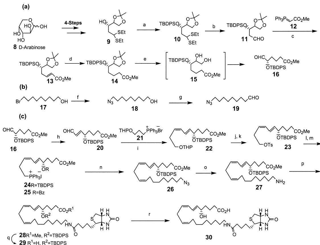
Scheme 4. Reagents and conditions: (a) tert -butylchlorodiphenylsilane, imidazole, \text{CH}_2\text{Cl}_2 , 0^\circ\text{C} to RT, 97%; (b) \text{H}_5\text{IO}_6 , ether, THF, 0^\circ\text{C} , 15 min, quant.; (c) benzene, reflux, 4 h, 85%; (d) \text{Pd-C}/\text{H}_2 , quant.; (e) \text{H}_5\text{IO}_6 , ether/THF, RT, 18 h, 92%; (f) \text{NaN}_3 , DMSO, 90^\circ\text{C} , 99%; (g) PCC, \text{CH}_2\text{Cl}_2 , 0^\circ\text{C} to RT, 77%; (h) (triphenylphosphoranylidene)-acetaldehyde, benzene, reflux, 78%; (i) LiHMDS, 20 , -78^\circ\text{C} to RT, 90%; (j) 1N HCl, THF: \text{H}_2\text{O} (9:1), RT, 40 h, 48%; (k) p -TsCl, Py, 0^\circ\text{C} to RT, 82%; (l) NaI, acetone, 65^\circ\text{C} , 99%; (m) \text{Ph}_3\text{P} , \text{CH}_3\text{CN} , 65^\circ\text{C} , 99%; (n) LiHMDS, 19 , -78^\circ\text{C} to RT, 36%; (o) \text{Ph}_3\text{P} , THF/ \text{H}_2\text{O} , RT, 88%; (p) (+)-biotin, EDCI, HOBT, \text{NaHCO}_3 , DMF, RT, 76%; (q) 1N NaOH (aq), MeOH, 92%; (r) THF, TBAF: \text{HOAc} (1:1), RT, 80 h, 74%
