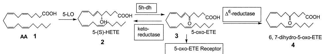
Scheme 1. Four proteins involved in the biosyntheses, metabolism and biological activity of 5-oxo-EETE
