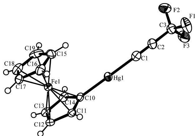
Figure 2. Representation of the molecular structure of \text{FcHgC}\equiv\text{CCF}_3 ( 2 ) (30% thermal ellipsoids). Selected bond distances (Å) and angles (deg): \text{Hg1}-\text{C1} 2.050(6), \text{Hg1}-\text{C10} 2.039(6), \text{C1}-\text{C2} 1.183(9), \text{C2}-\text{C3} 1.450(9), \text{C3}-\text{F1} 1.335(8), \text{C3}-\text{F2} 1.344(8), \text{C3}-\text{F3} 1.341(8), \text{Hg1}-\text{C1}-\text{C2} 178.1(6), \text{C10}-\text{Hg1}-\text{C1} 179.4(2), \text{C1}-\text{C2}-\text{C3} 175.9(7), \text{C2}-\text{C3}-\text{F1} 112.9(6), \text{C2}-\text{C3}-\text{F2} 112.5(6), \text{C2}-\text{C3}-\text{F3} 112.7(5).
