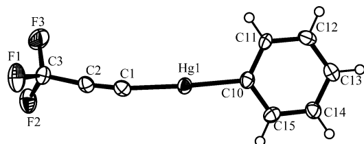
Figure 1. Representation of the molecular structure of \text{PhHgC}\equiv\text{CCF}_3 ( 1 ) (30% thermal ellipsoids). Selected bond distance (Å) and angles (deg): \text{Hg1}-\text{C1} 2.029(9), \text{Hg1}-\text{C10} 2.052(9), \text{C1}-\text{C2} 1.192(13), \text{C2}-\text{C3} 1.465(13), \text{C3}-\text{F1} 1.327(11), \text{C3}-\text{F2} 1.344(12), \text{C3}-\text{F3} 1.336(11), \text{Hg1}-\text{C1}-\text{C2} 170.2(7), \text{C10}-\text{Hg1}-\text{C1} 175.3(3), \text{C1}-\text{C2}-\text{C3} 174.2(9), \text{C2}-\text{C3}-\text{F1} 114.7(7), \text{C2}-\text{C3}-\text{F2} 111.5(8), \text{C2}-\text{C3}-\text{F3} 112.2(8).
