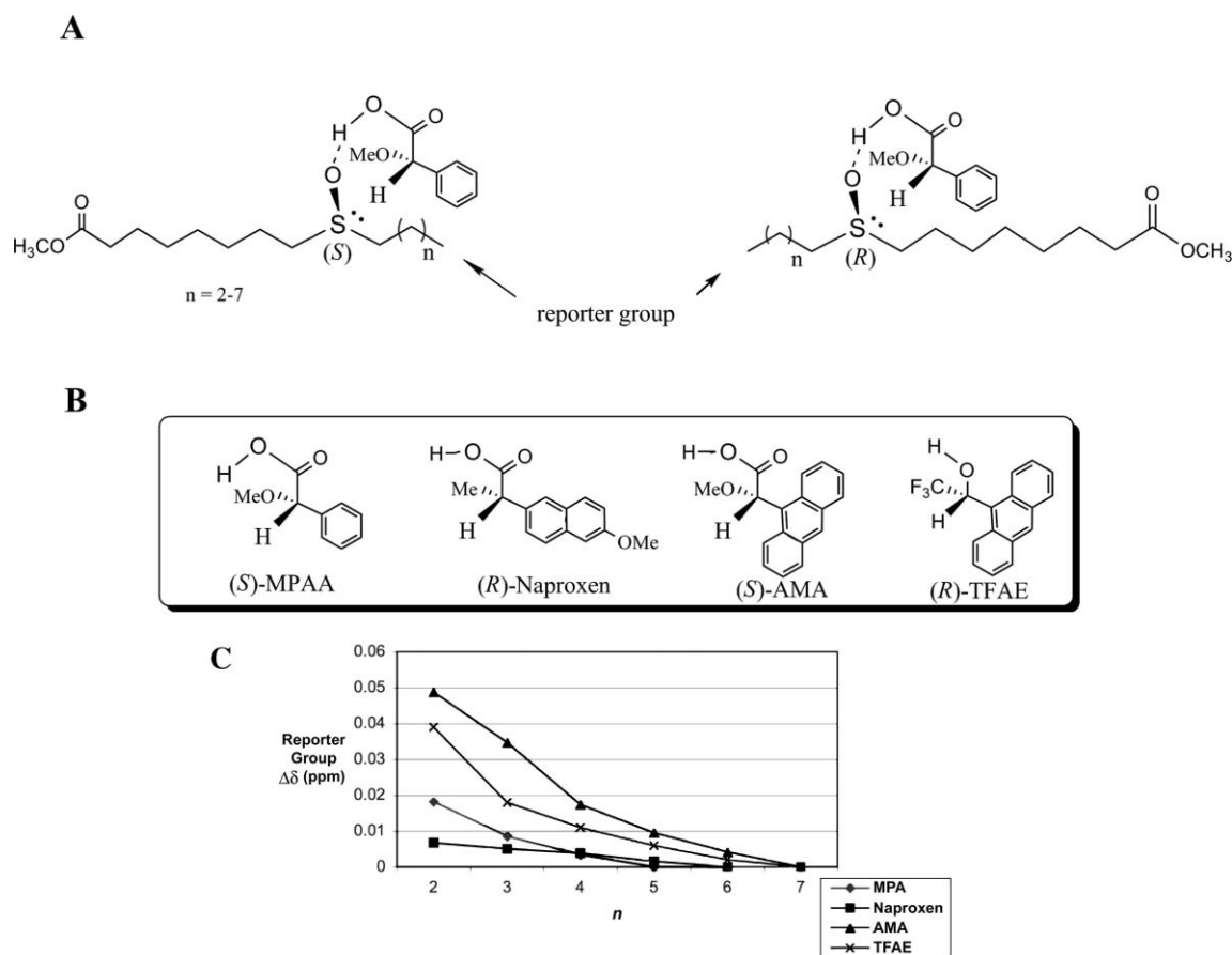
Fig. 1 (A) Pirkle-type complexation model featuring differential shielding effects of (S)-(+)-MPAA on ^1\text{H} NMR signals of a methyl reporter group; (B) various chiral solvating agents that are useful in probing stereochemistry of fatty acid sulfoxides; (C) magnitude of induced non-equivalence as a function of the number of methylene units ( n ) between the reporting group and C10 of 9-sulfoxide.
