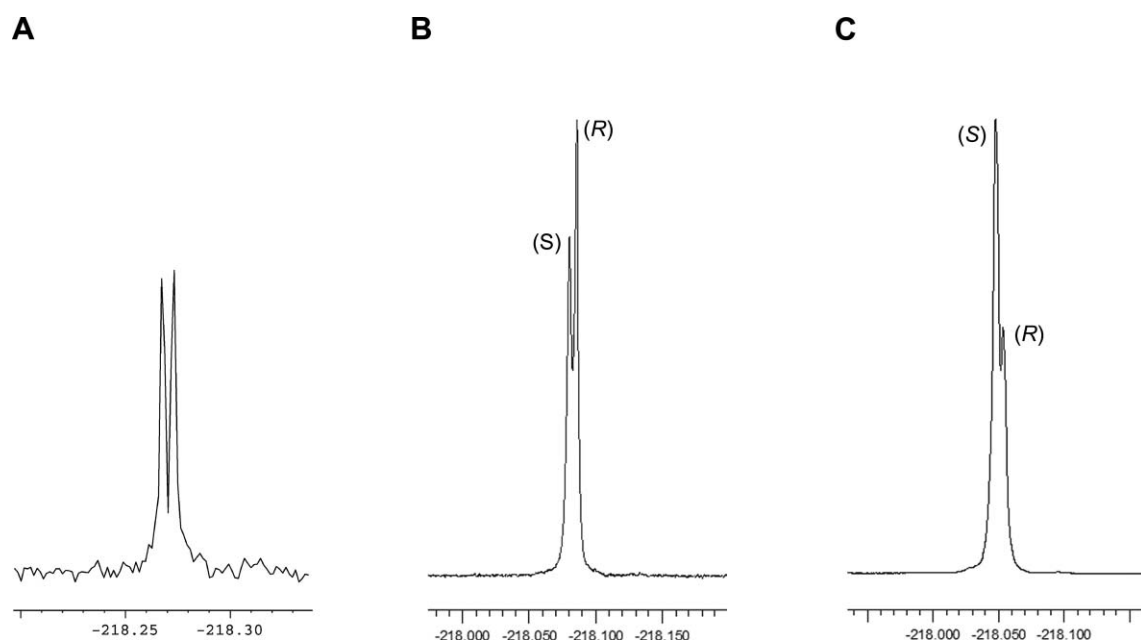
Fig. 3 ^1\text{H} -decoupled ^{19}\text{F} NMR signal of (A) racemic 18-fluoro-10-thiooctadecan-1-ol ( racemic -1); (B) ( R )-1 : ( S )-1, 2 : 1 mixture + ( R )-AMA; (C) ( R )-1 : ( S )-1, 1 : 2 mixture + ( R )-AMA.
