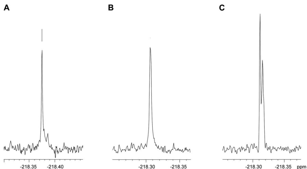
Fig. 2 ^1\text{H} -decoupled ^{19}\text{F} NMR signal of (A) enzymatically generated sample of 18-fluoro-10-thiaoctadecan-1-ol ( bio-1 ); (B) ( bio-1 ) + ( R )-AMA (50 mg \text{mL}^{-1} ); (C) ( bio-1 ) spiked with racemic 1 + ( R )-AMA (50 mg \text{mL}^{-1} ).
