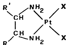
Scheme 1. Cisplatin analogues used in this work. The diamines (diam) and their abbreviations are: R = R' = H, ethylenediamine, en; R = H, R' = CH 3 , (R)- and (S)-propane-1,2-diamine, pn; R = R' = CH 3 , (R,R)-, (S,S)-, and meso -butane-2,3-diamine, bn; R = H, R' = C 6 H 5 , (R)-1-phenylethylenediamine, pen; R = R' = C 6 H 5 , (R,R)-, (S,S)-, and meso -1,2-diphenylethylenediamine, dpen; also diam = (R,R)-, (S,S)-, and meso -cyclohexane-1,2-diamine; chxn. X = Cl for [diamPtCl 2 ]; and X = H 2 O for [diamPt(H 2 O) 2 ]SO 4 .
