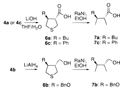
Scheme 3. Cleavage of the Camphorsultam Auxiliary and Subsequent Reductive Desulfurization
