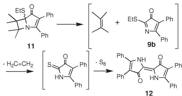
Scheme 3. Formation of Bipyrrrolinone 12 from Azabicyclo[3.2.0]hept-2-en-4-one 11
