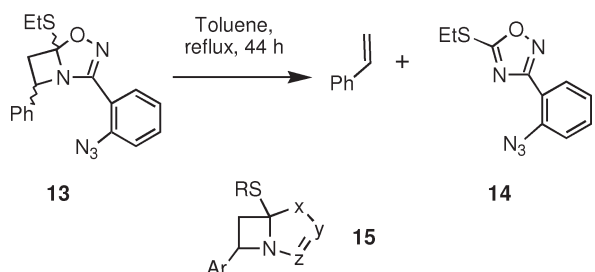
Scheme 4. Formation of 1,2,4-Oxadiazole 14 from Oxadiazabicyclo[3.2.0]heptene 13
