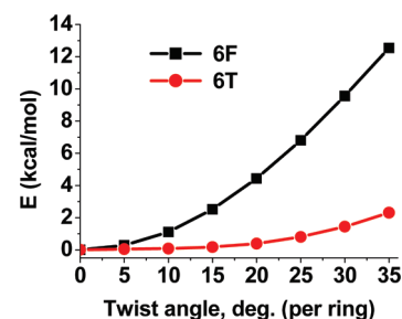
Figure 3. Calculated [B3LYP/6-31G(d)] relative energies required for spiral twisting of 6F and 6T as functions of twist angle.
