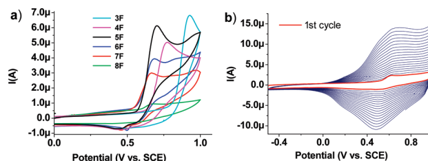
Figure 4. (a) CV of 3F – 8F in PC with 0.1 M TBABF 4 (scan rate 50 mV/s) and (b) repetitive CV scans of 6F in 1,2-dichloroethane with 0.1 M TBABF 4 (scan rate 100 mV/s). \text{Fc}/\text{Fc}^+ = 0.34 V vs SCE under these conditions.
