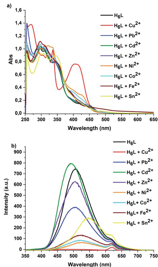
Fig. 3 (a) UV-vis spectra of H 6 L + M 2+ , (b) fluorescence spectra of H 6 L + M 2+ ( \lambda_{\text{ex}} = 310 nm, slit; 10 nm/10 nm) of H 6 L (25 \mu M) and M 2+ (25 \mu M) in DMSO.
