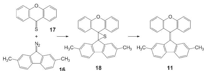
Scheme 1. Synthesis of 9-(2,7-dimethyl-9 H -fluoren-9-ylidene)-9 H -xanthene ( 11 ).
