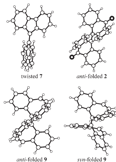
Figure 1. Molecular structures of 9,9'-bi-(9 H -fluoren-9-ylidene) ( 7 ), 9,9'-bi-(9(10 H )-anthracenylidene)-10,10'-dione ( 2 ), and 5,5'-bi-(5 H -dibenzo[ a,d ]cyclohept-5-ylidene) ( 9 ), determined by X-ray crystallography.
