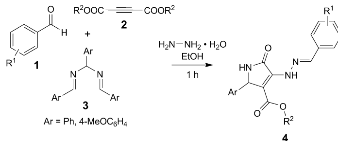
Scheme 1. Synthesis of 2-Aryl-2,5-dihydro-5-oxo-4-[2-(phenylmethylenidene)hydrazino]-1H-pyrroles
