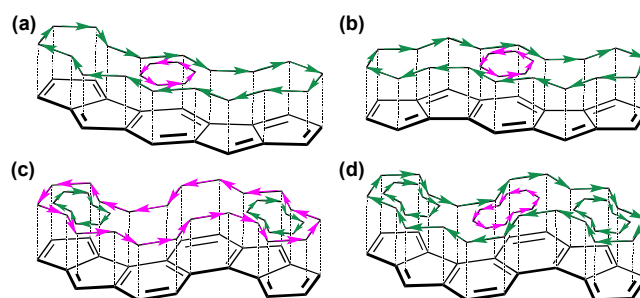
Figure 5. Scheme of induced ring currents from NICS-XY-scan results for (a) bispentalene 1 , (b) bispentalene 2 , (c) one possibility for bispentalene 3 , and (d) the second possibility for bispentalene 3 . Substituents and the small local paratropic currents at the five-membered rings (Figure S45, Supporting Information) are omitted for clarity.
