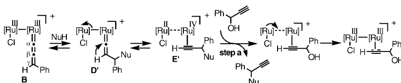
Scheme 12. The possibility of the synergistic effects of two ruthenium atoms.
