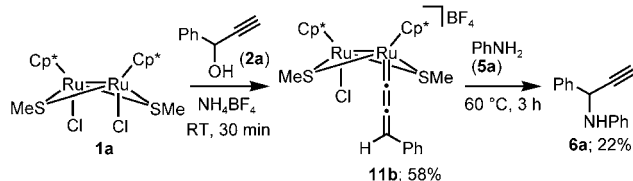
Scheme 4. Stoichiometric reaction of the allenylidene complex 11b with aniline.
