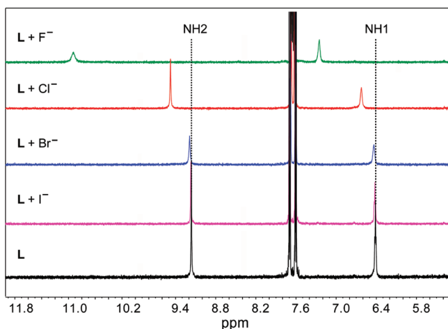
Figure 1. Partial ^1\text{H} NMR spectra of L (2 mM) in the absence and presence of an anion showing two NH peaks in \text{DMSO}-d_6 . An equivalent amount of [n\text{-Bu}_4\text{N}]^+\text{X}^- was added to the ligand solution.
