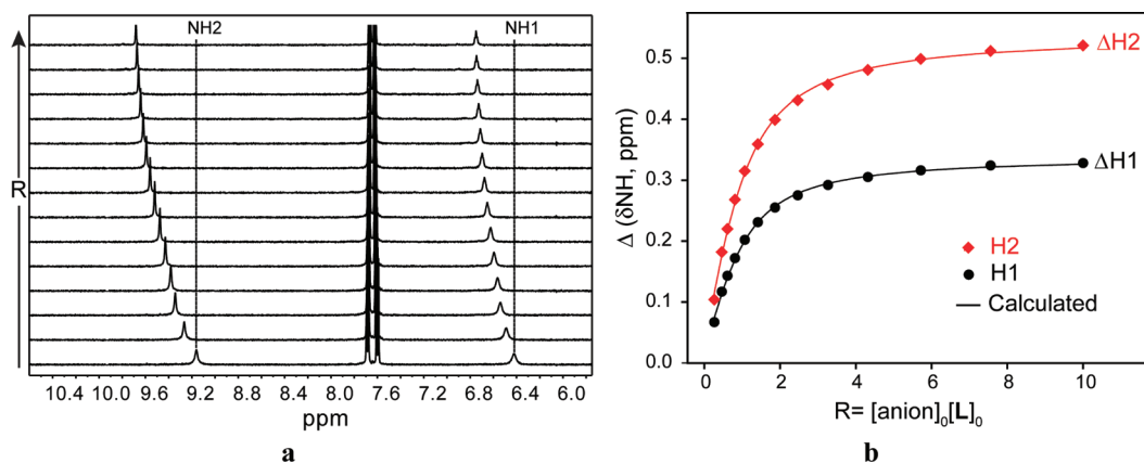
Figure 2. (a) Partial ^1\text{H} NMR titration of L (2 mM) with an increasing addition of [n\text{-Bu}_4\text{N}]^+\text{Cl}^- (20 mM) in \text{DMSO}-d_6 . (b) ^1\text{H} NMR titration curves of L with [n\text{-Bu}_4\text{N}]^+\text{Cl}^- in \text{DMSO}-d_6 showing the net changes in the chemical shifts of NH (H1 = \text{CH}_2\text{NHCO} and H2 = \text{CONHAr} ).
