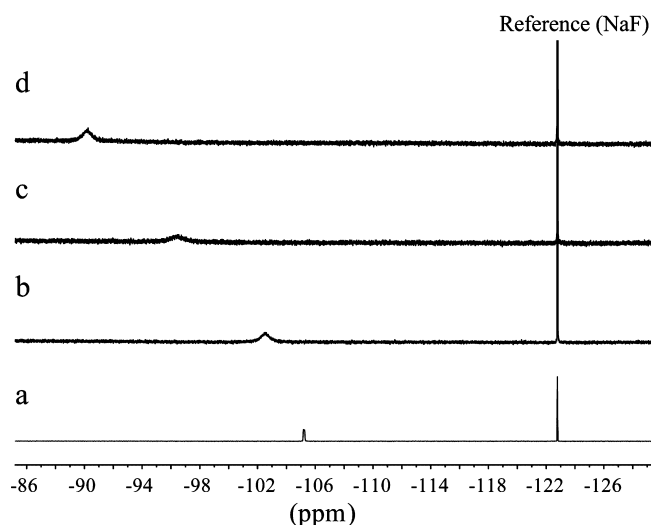
Figure 3. Partial ^{19}\text{F} NMR spectra of [n\text{-Bu}_4\text{N}]^+\text{F}^- in \text{DMSO}-d_6 at room temperature, showing the downfield shift of \text{F}^- resonance upon the gradual addition of L . (a) Free [n\text{-Bu}_4\text{N}]^+\text{F}^- ( \delta_{\text{F}} = -105.2 ppm), (b) [n\text{-Bu}_4\text{N}]^+\text{F}^- + 0.25 equiv of L ( \delta_{\text{F}} = -102.5 ppm), (c) [n\text{-Bu}_4\text{N}]^+\text{F}^- + 0.50 equiv of L ( \delta_{\text{F}} = -96.4 ppm), and (d) [n\text{-Bu}_4\text{N}]^+\text{F}^- + 1.0 equiv of L ( \delta_{\text{F}} = -90.1 ppm).
