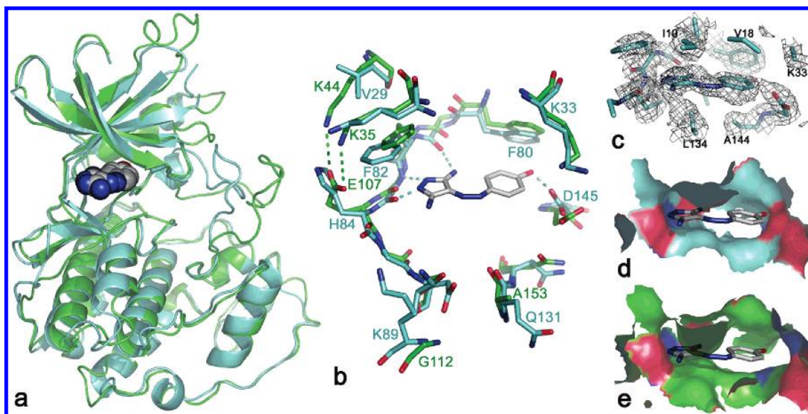
Figure 3. Crystal structure of CDK2 complex with 31b . (a) The experimentally determined 3D structure of CDK2 (cyan) aligned with the modeled structure of CDK9 (green); the ligand is shown as a space-filling CPK representation. (b) Details of the interactions between ligand and residues of the ATP-binding pocket, indicated with broken lines. (c) Observed electron density around the bound inhibitor 31b . The protein surfaces within 4 Å of the ligand are shown for CDK2 (d) and CDK9 (e), respectively.
