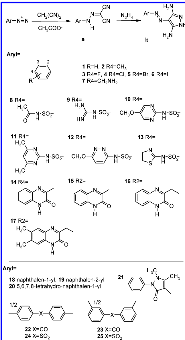
Scheme 1. Synthesis of 4-Arylazo-3,5-diamino-1H-pyrazoles
