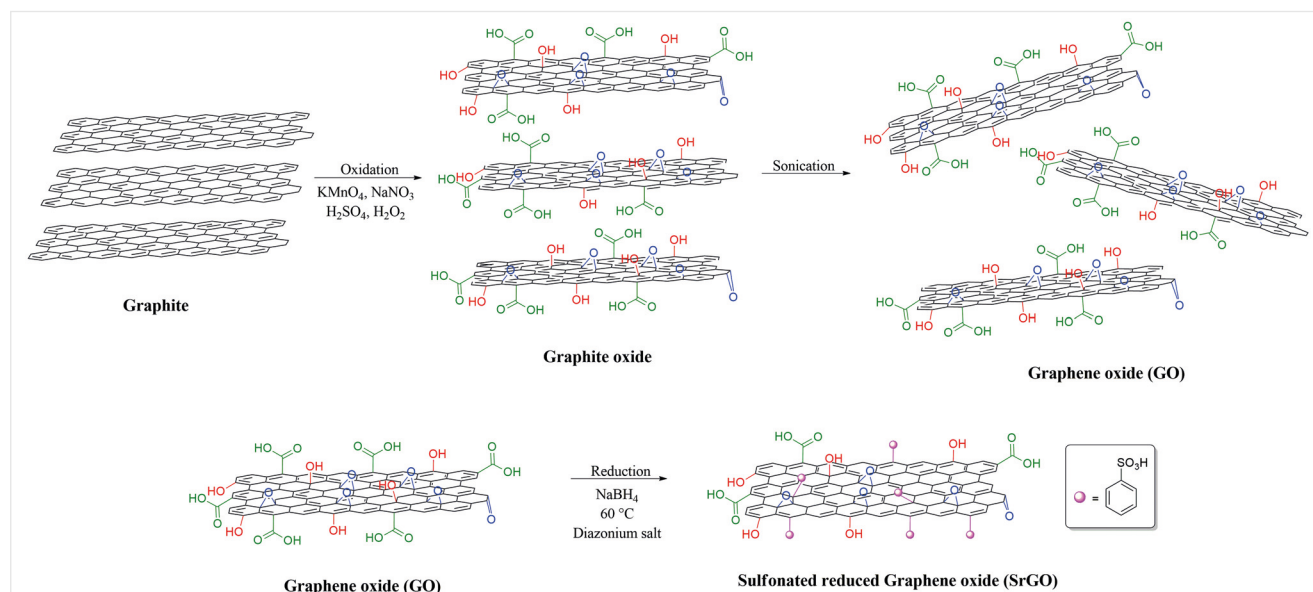
Figure 1 Schematic diagram for the preparation of GO and SrGO
