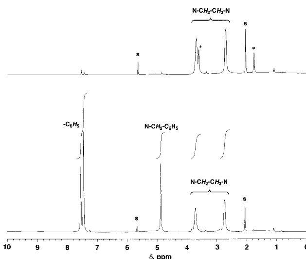
Figure 12. 500 MHz ^1\text{H} NMR spectra of (top) [(d_{21}\text{-L}^{\text{Bn}_3}\text{Cu})_2(\mu\text{-O})_2](\text{ClO}_4)_2 and (bottom) [(\text{L}^{\text{Bn}_3}\text{Cu})_2(\mu\text{-O})_2](\text{ClO}_4)_2 in 2:1 (\text{CD}_3)_2\text{CO}/\text{CD}_2\text{Cl}_2 at -75 °C (s denotes peaks due to residual hydrogen atoms in the solvents; * indicates THF impurity present in the Cu(I) precursor).
