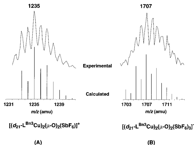
Figure 3. Experimental (top) and calculated (bottom) peak envelopes in the positive ion (A) and negative ion (B) electrospray mass spectra of [(d_{21}\text{-L}^{\text{Bn}_3}\text{Cu})_2(\mu\text{-O})_2](\text{SbF}_6)_2 in \text{CH}_2\text{Cl}_2 .
