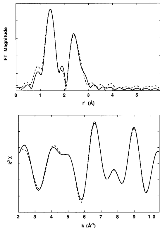
Figure 11. EXAFS data ( k = 2\text{--}10.5 Å ^{-1} ) (---) and simulations (—) for [(\text{L}^{\text{iPr}_3}\text{Cu})_2(\mu\text{-O})_2](\text{ClO}_4)_2 : (top) r' -space spectrum; (bottom) k -space spectrum.
