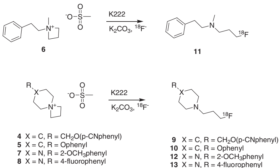
Scheme 2. Radiosynthesis
