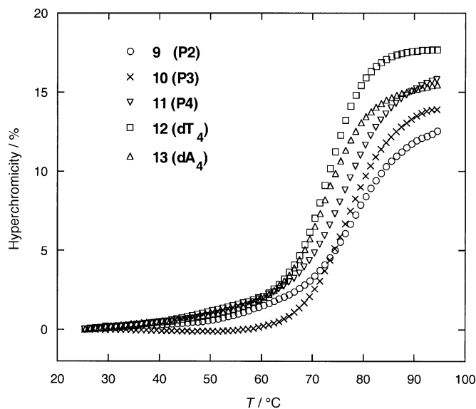
Fig. 1. Melting curves of the hairpin mimics 9–11 in comparison with the control hairpins 12 and 13 . Conditions: oligonucleotides 2.5 \mu\text{M} , 100 mM NaCl, 10 mM Tris \cdot HCl, pH 7.5.
