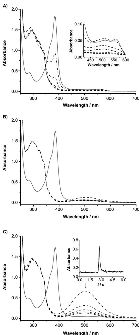
Figure 1. Spectral changes of HNTTM' ( 60 \mu\text{mol L}^{-1} ) in the absence (solid line) and presence (dashed line) of the hydroxylated hybrid 11b ( 60 \mu\text{mol L}^{-1} ) in chloroform/methanol with various volume ratios of 49:1 (A), 9:1 (B), and 4:1 (C) at 25^\circ\text{C} (the interval: 1 min). The inset in A shows the enlargement of absorbance in the range \lambda = 420\text{--}600 \text{ nm} . The inset in C shows decay of HNTTM' ( 30 \mu\text{mol L}^{-1} ) at 387 \text{ nm} in the presence of 11b ( 30 \mu\text{mol L}^{-1} ) in chloroform/methanol (4:1, v/v) using the stopped-flow UV/Vis spectroscopy at 25^\circ\text{C} .
