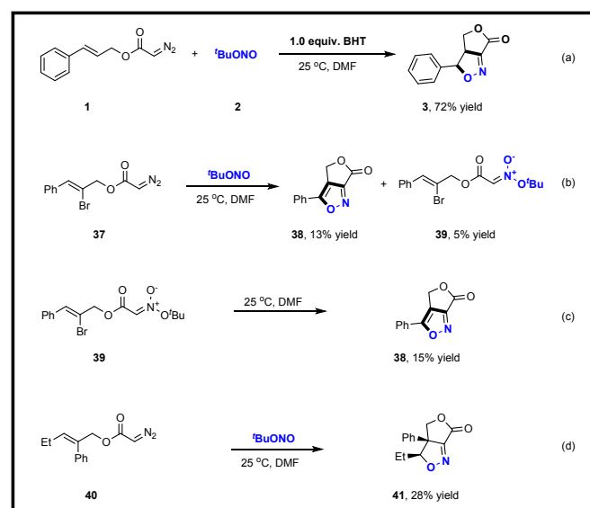
Scheme 3 Probe for the possible mechanism.
