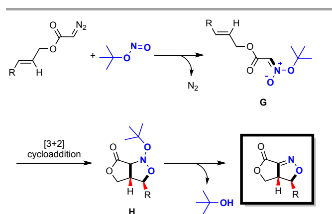
Scheme 4 Proposed catalytic cycle.
