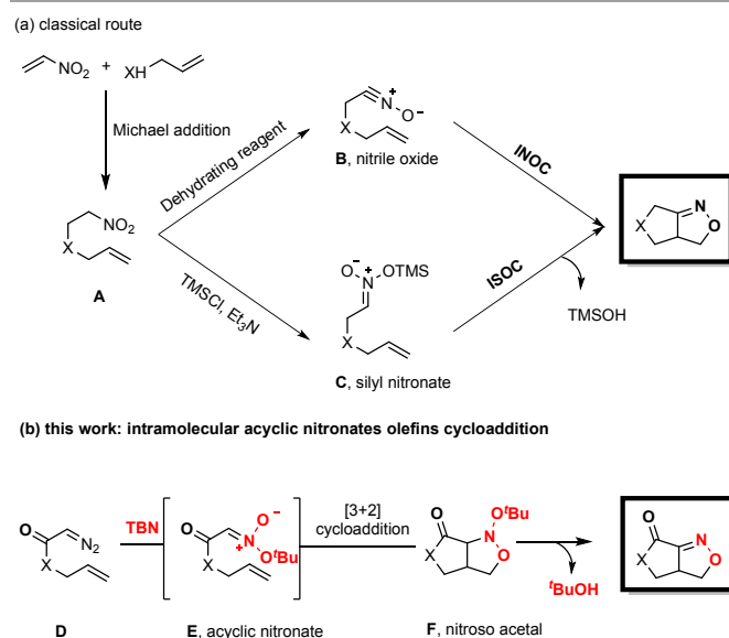
Scheme 1 Synthesis of isoxazoline fused bicyclic compounds.
