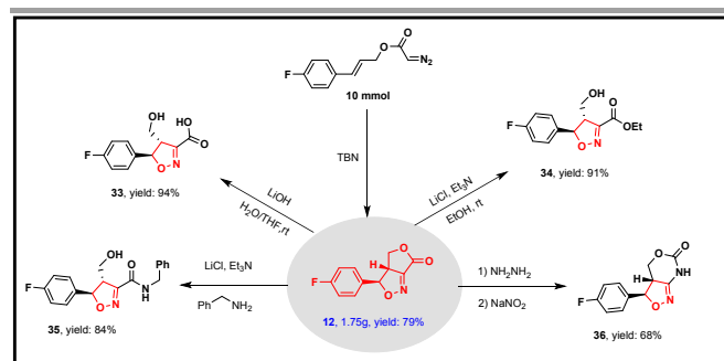
Scheme 2 Synthetic utility.
