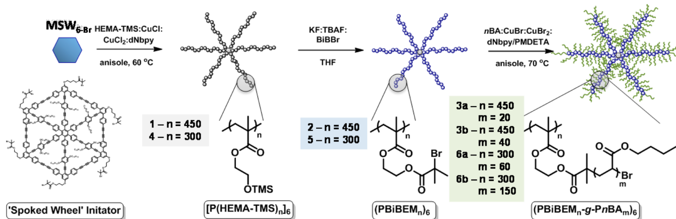
Scheme 1. Synthesis of Star-like Bottlebrushes with Hexa-arm ATRP Initiator \text{MSW}_{6-\text{Br}} via Double “Grafting-from” Approach
