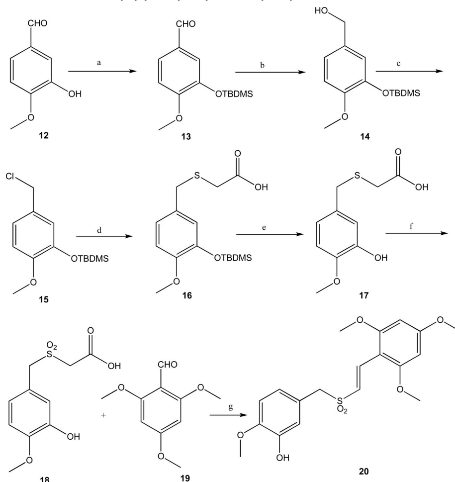
Scheme 3. Synthesis of ( E )-2,4,6-(Trimethoxystyryl)-3-hydroxy-4-methoxybenzylsulfone a
