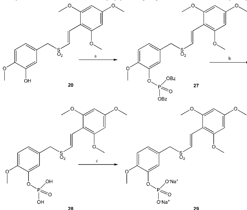
Scheme 5. Method for the Synthesis of ( E )-2,4,6-(Trimethoxystyryl)-3- O -phosphate Disodium 4-Methoxybenzylsulfone a
