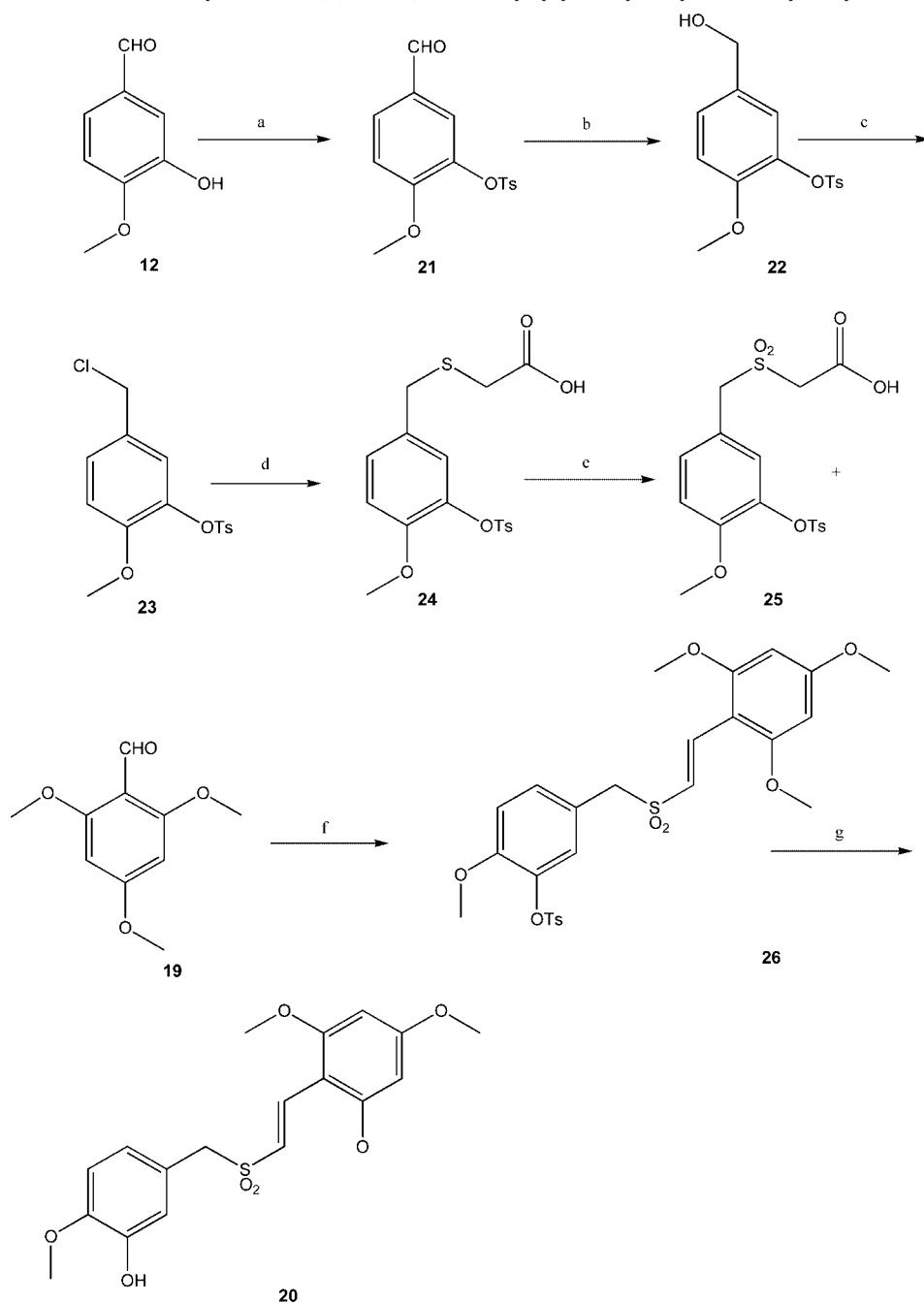
Scheme 4. Alternative Method for the Synthesis of (E)-2,4,6-(Trimethoxystyryl)-3-hydroxy-4-methoxybenzylsulfone a
