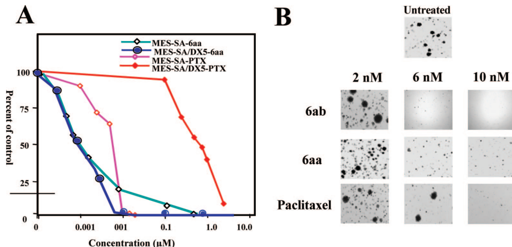
Figure 1. Antitumor effects of 6aa . (A) 6aa inhibits the growth of parental (MES-SA) and paclitaxel-resistant (MES-SA/DX5) cell lines with equal efficiency. The parental uterine sarcoma cells and the MDR positive (MES-SA/DX5) cells were plated into six-well dishes and treated with various concentrations of 6aa and paclitaxel for 96 h. The number of viable cells from duplicate plates was determined by trypan blue exclusion. (B) Shown are results from soft agar assays. MIA-PaCa-2 cells ( 1.0 \times 10^5 ) were plated in soft agar containing various concentrations of each compound in triplicate. After 3 weeks of growth, the plates were stained for 48 h using 0.05% nitroblue tetrazolium solution. Representative plates were photographed using an Olympus stereoscope mounted with a Sony digital camera system (DKC5000, Sony Inc.).
