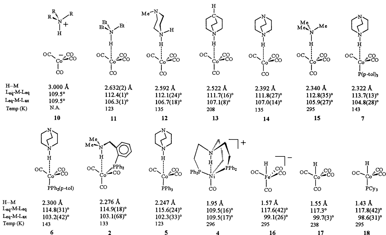
Scheme 1. Structures whose geometries were used in the Structure Correlation study to determine the geometric changes that define the pathway for protonation of \text{Co(CO)}_3\text{L}^- . Average values \langle r \rangle are listed for the angles with esds ( \sigma ) representing the scatter in these angles (i.e. \sigma = [\sum_i (\langle r \rangle - r_i)^2 / (n - 1)]^{1/2} , where r_i = i th observation, n = number of observations). These e.s.d.s do not necessarily correlate with those of individual angles. H–M distances for 12–15 , 7 , 6 , 2 , and 5 are calculated after normalizing the X-ray determined N–H distance to 1.054 Å, as determined by neutron diffraction in 11 . Original references for the X-ray structures are 10 [model geometry, this work], 11 ([21], neutron diffraction), 12 [3c], 13 [3e], 14 [3f], 15 [4a], 7 [3f], 6 [3f], 2 (this work), 5 [3e], 4 [4b], 16 [19], 17 ([17], electron diffraction), 18 [18]. See also Ref. [22] for reports of the synthesis and IR characterization, but not crystal structures, of \text{HCo(CO)}_3\text{PPh}_3 , \text{HCo(CO)}_3\text{P(OPh)}_3 and \text{Et}_3\text{NH}^+\text{Co(CO)}_3\text{PPh}_3^- .
