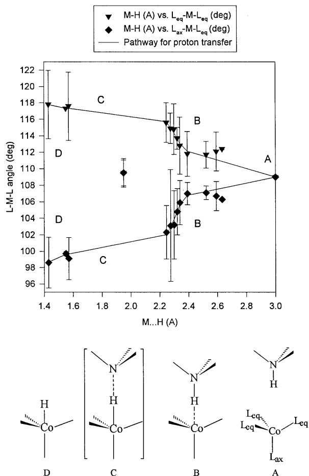
Fig. 3. Structure Correlation study, modelling the pathway for protonation of \text{Co}(\text{CO})_3\text{L}^- anion at the metal center. Error bars on \text{L--M--L} angles at 1\sigma level (see Scheme 1 for calculation of \sigma ).
