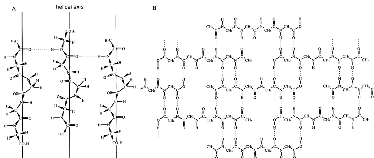
Fig. 5 PGII(helical)-type (A) and PGI( \beta -sheet)-type (B) structural models for the N -acetylglutamine tetramer. The dotted lines represent hydrogen bonding.
