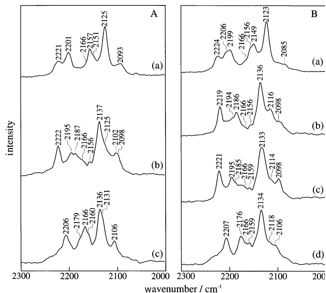
Fig. 4 Raman spectra of selectively C-deuterated PGI-type N -acetylglutamine oligomers in the solid state in the \text{CD}_2 stretch region. [A, Trimers: (a) G1D3-B; (b) G2D3-B; (c) G3D3-B. B, Tetramers: (a) G1D4-B; (b) G2D4-B; (c) G3D4-B; (d) G4D4-B].
