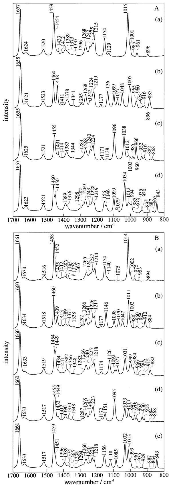
Fig. 3 Raman spectra of undeuterated and selectively C-deuterated PGI-type N -acetylglutamine oligomers in the solid state in the 800–1700 \text{cm}^{-1} region. [A, Trimers: (a) undeuterated; (b) G1D3-B; (c) G2D3-B; (d) G3D3-B. B, Tetramers: (a) undeuterated; (b) G1D4-B; (c) G2D4-B; (d) G3D4-B; (e) G4D4-B].
