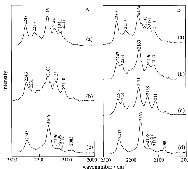
Fig. 2 Raman spectra of selectively C-deuteriated PGII-type N-acetylglycine oligomers in the solid state in the CD 2 stretch region. [A, Trimers (a) G1D3-A; (b) G2D3-A; (c) G3D3-A. B, Tetramers: (a) G1D4-A; (b) G2D4-A; (c) G3D4-A; (d) G4D4-A].
