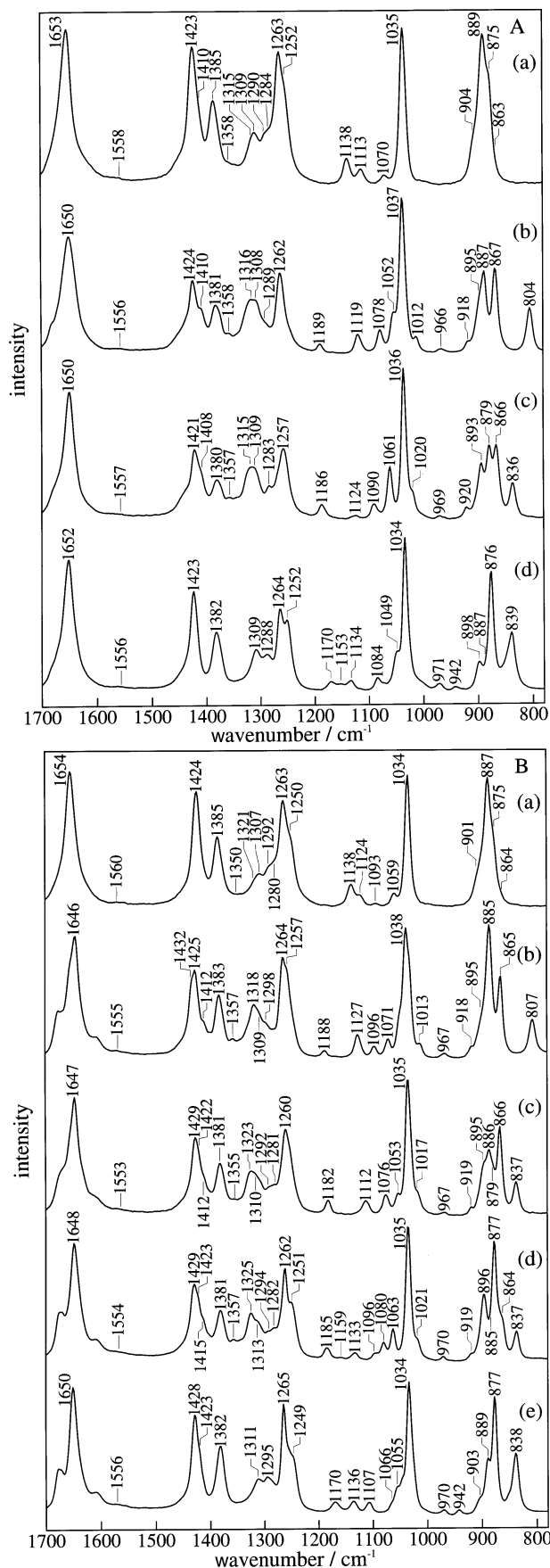
Fig. 1 Raman spectra of undeuterated and selectively C-deuterated PGII-type N -acetylglycine oligomers in the solid state in the 800–1700 \text{cm}^{-1} region. [A, Trimers: (a) undeuterated; (b) G1D3-A; (c) G2D3-A; (d) G3D3-A. B Tetramers: (a) undeuterated; (b) G1D4-A; (c) G2D4-A; (d) G3D4-A; (e) G4D4-A].
