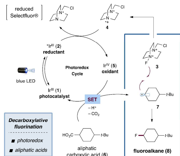
Scheme 1. Mechanism for Decarboxylative Fluorination.
