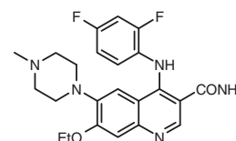
Figure 1. 3-Amidoquinoline AZ683.
