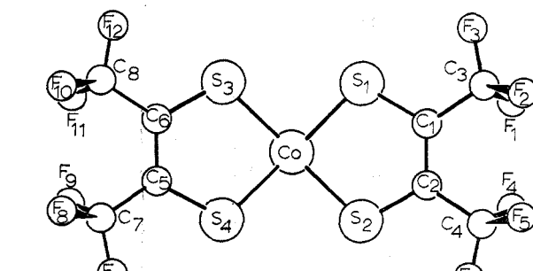
Figure 1.—Molecular structure and numbering system for half of the dimeric molecule.
