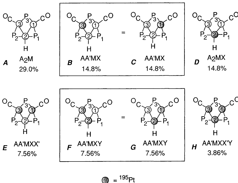
Figure 2. ^{31}\text{P}\{^1\text{H}\} NMR spectrum ( \text{C}_6\text{D}_6 , 293 K) of complex 2: (upper trace) experimental; (lower trace) simulated.
