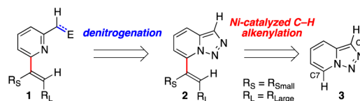
Scheme 1. Synthesis of 2,6-Disubstituted Pyridines from C–H Bond Functionalization–Denitrogenation of Triazolopyridines
