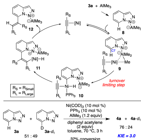
Scheme 2. Potential Catalytic Cycle
