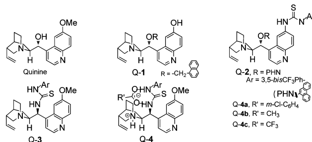
Figure 1. Structure of cinchona alkaloid catalysts.
