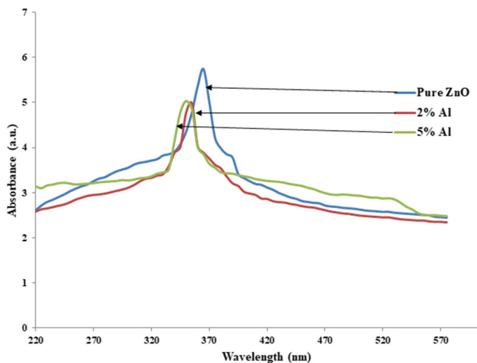
Fig. 6 UV absorption analysis of pure ZnO and Al-doped ZnO nanostructures
