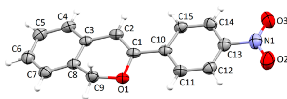
Figure 2. ORTEP-type view of the structure of 2p .
