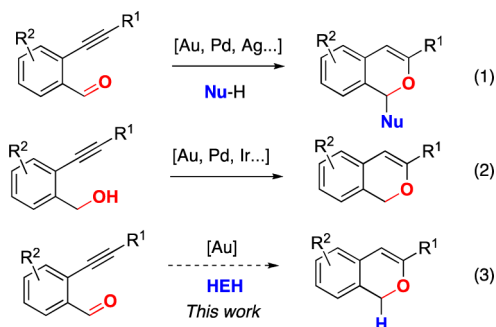
Scheme 1. [M]-Catalyzed Access to 1 H -Isochromenes
