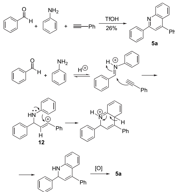
Scheme 6. \text{TfOH} -catalyzed three-component reaction.
