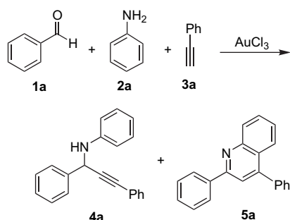
Scheme 2. AuCl 3 -catalyzed three-component reaction of aldehydes 1a , amine 2a , and terminal alkyne 3a .
