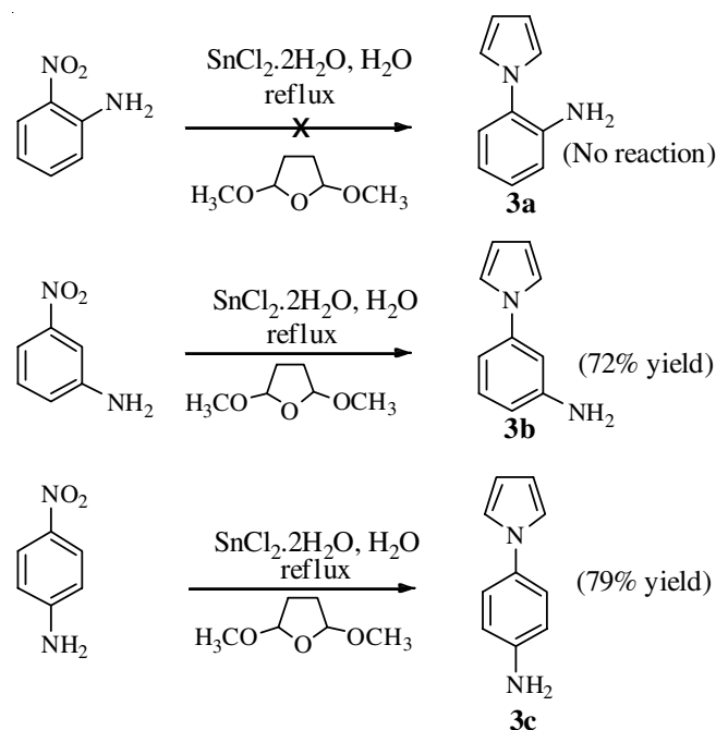
Scheme-II: Preparation of substituted pyrrole-chemoselectivity
