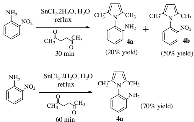
Scheme-III: Preparation of pyrrole from o -nitro aniline
