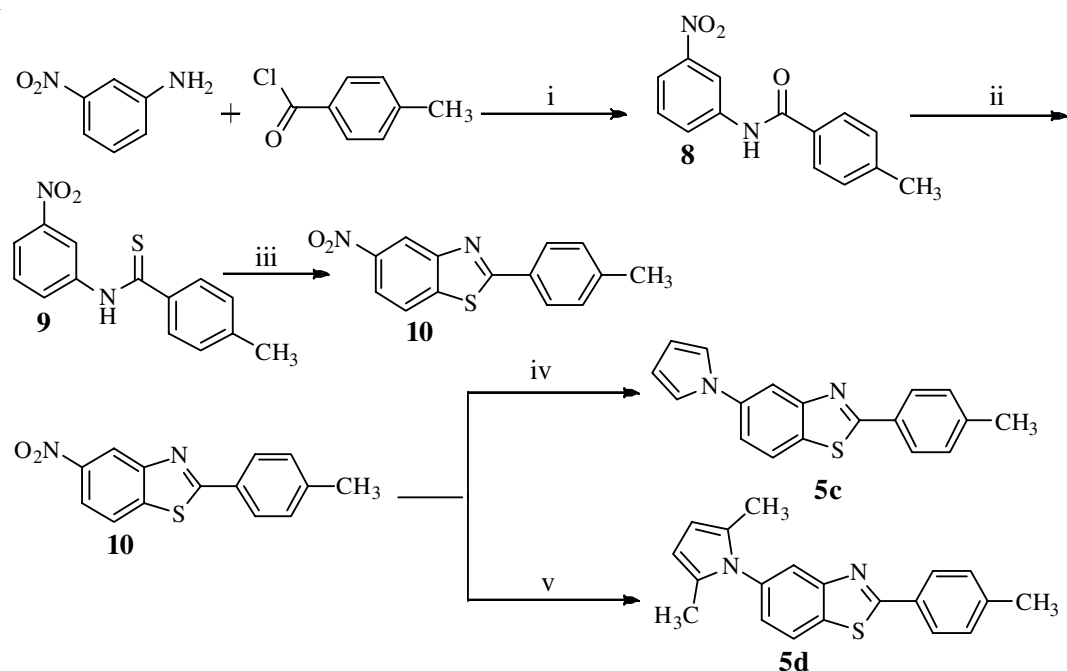
Scheme-VI: Synthesis of benzoxazole-pyrrole hybrid molecule 5a
