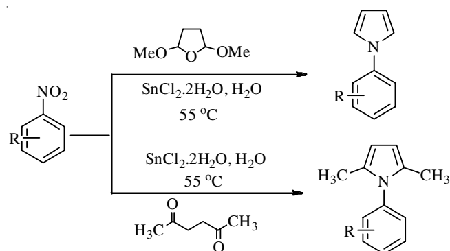
Scheme-I: Synthesis of pyrrole from nitrobenzene
