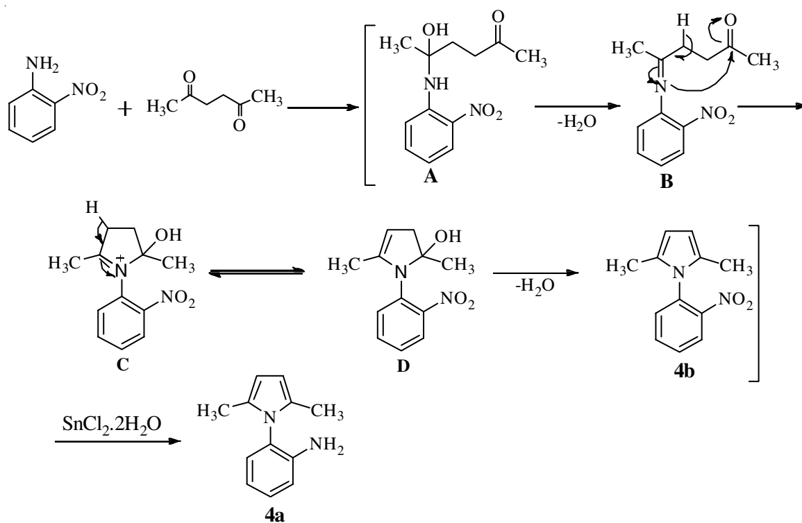
Scheme-IV: Plausible mechanism for formation of 4a
