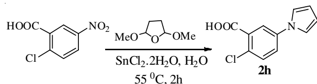
Scheme-V: Synthesis of pyrrole derivative NB-64
