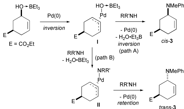
Scheme 1 Plausible reaction mechanism for allylic alkylation of N -methylaniline promoted by Pd-Et 3 B.
