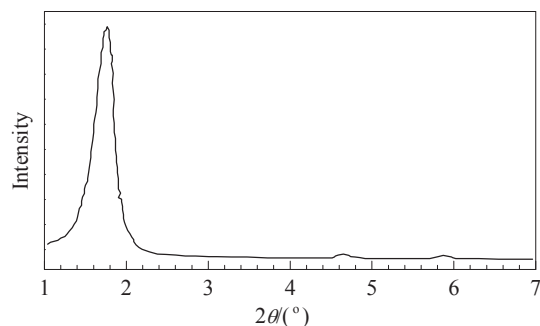
Fig. 2. XRD pattern of Zr-MCM-41.
