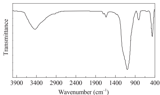
Fig. 1. FT-IR spectrum of the calcined Zr-MCM-41.
