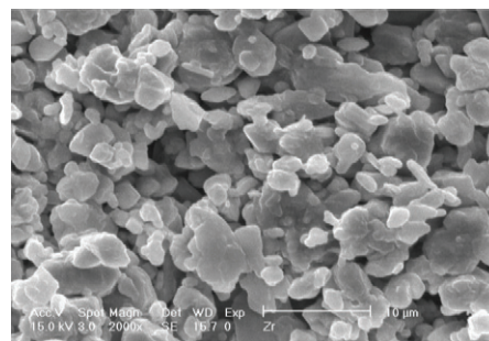
Fig. 3. SEM micrograph of the freshly activated Zr-MCM-41.
