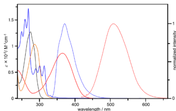
Figure 1. UV–vis (solid line) and fluorescence (dashed line) spectra of unsymmetrically functionalized germafluorene derivatives 2a (black), 2d (yellow), 2f (blue), and 6 (red) in CH_2Cl_2 ( 8 \times 10^{-6} ) at 25 °C.
